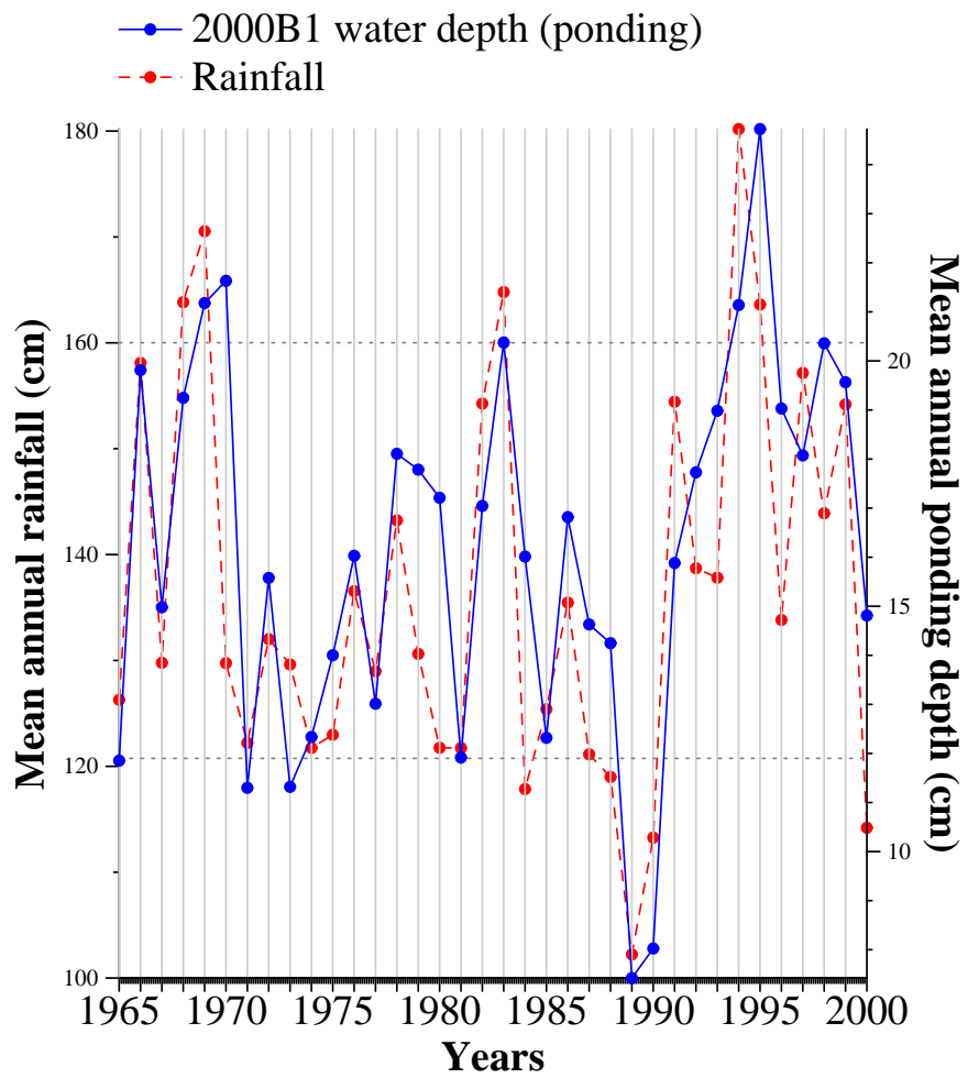
Comparison of mean annual rainfall with 2000B1 mean annual ponding depth over the SFWMM model area.
