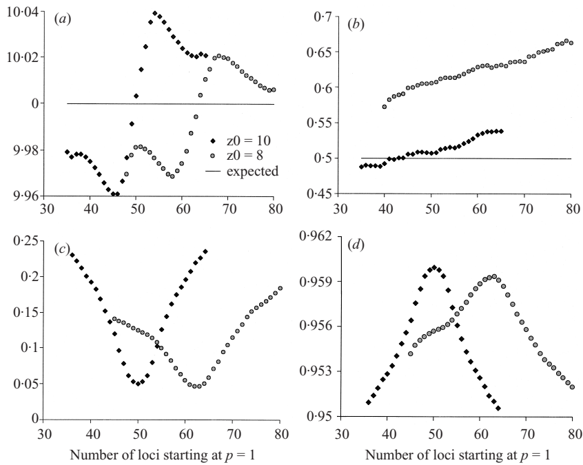
Fig. 1. Mutation–selection balance equilibrium for a phenotypically plastic trait. Mean reaction norm height, mean reaction norm slope, mean fitness and genotypic variance depend upon the number of loci starting at p_i = 1 . Selection on reaction norm height overrules selection on slope as the allelic values for height are much larger. Alternative equilibria for mean genotypic value occur. Variation in the environment equals \text{var}(x) = 1 . Allelic values are \alpha_i = z_0/n \cdot (0.5 + U_{x,i}) and \beta_i = z_1/n \cdot (0.5 + U_{\beta,i}) (the parameter a = 1.0 ). Averages of five runs. (A) Mean height \bar{g}_0 ; (B) mean slope \bar{g}_1 ; (C) genetic variance G^* = G_0^* + G_1^* \text{var}(x) ; (D) mean fitness.
